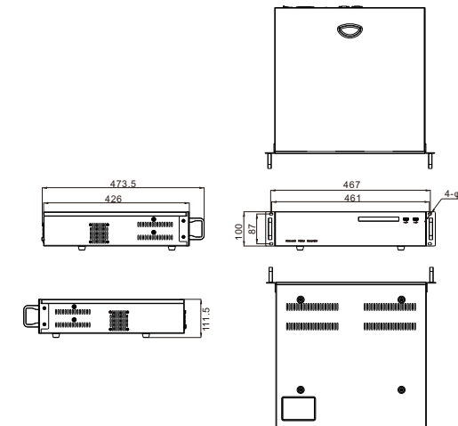
Figure 2-1 Dimensions (Unit:mm)
