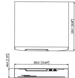
Figure 2-1 Dimensions (Unit:mm)
